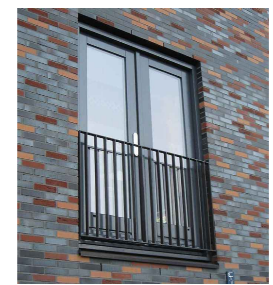
Powder coated metal railing to match balconies, fixed between reveals of opening.
